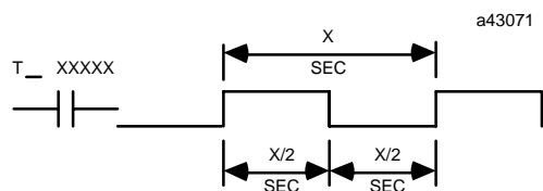
Figure 2.6 – Time–Tick Contact Timing Diagram
