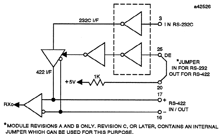
Figure 2-8. Port 1, RS-232C, Example Wiring Connection
