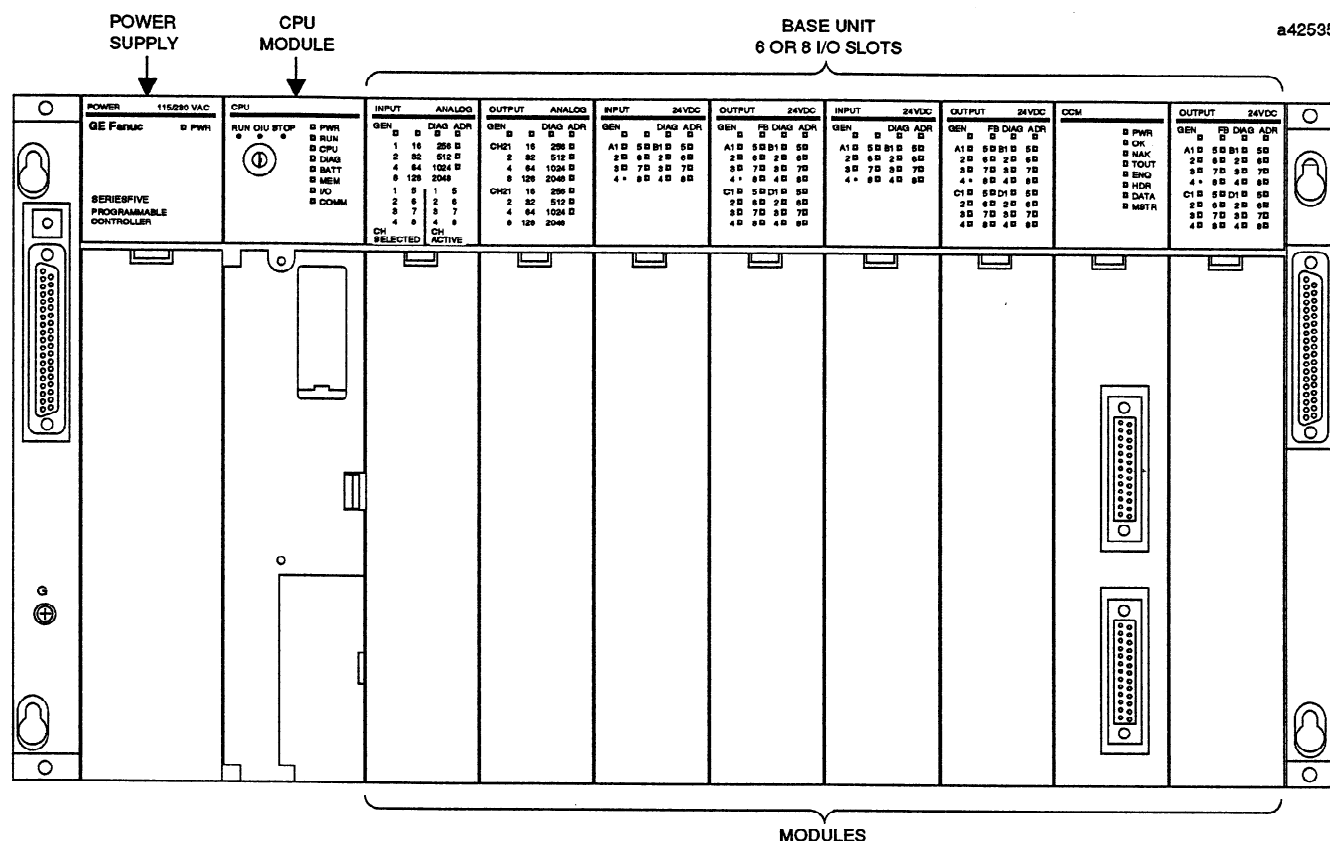
Figure 2-12. Series Five PLC Rack
