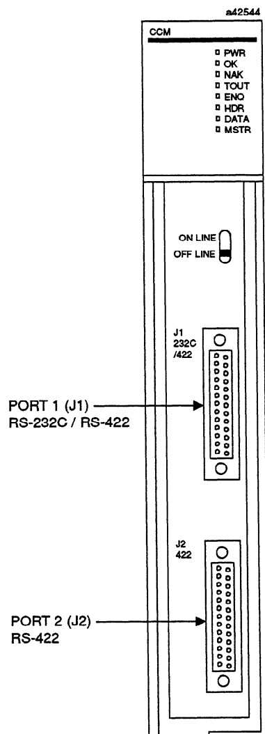
Figure 2-5. Communication Control Module (CCM) Front Panel
