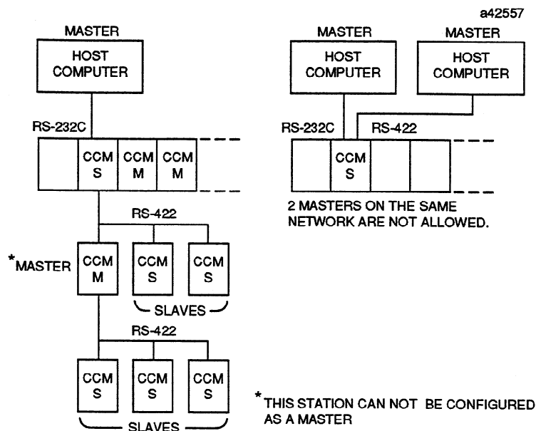
Figure 2-20. Illegal Network (Multi - Master Stations)
