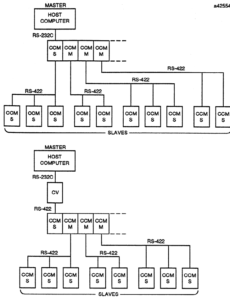
Figure 2-18. Complex Networks (Multiple Masters)
