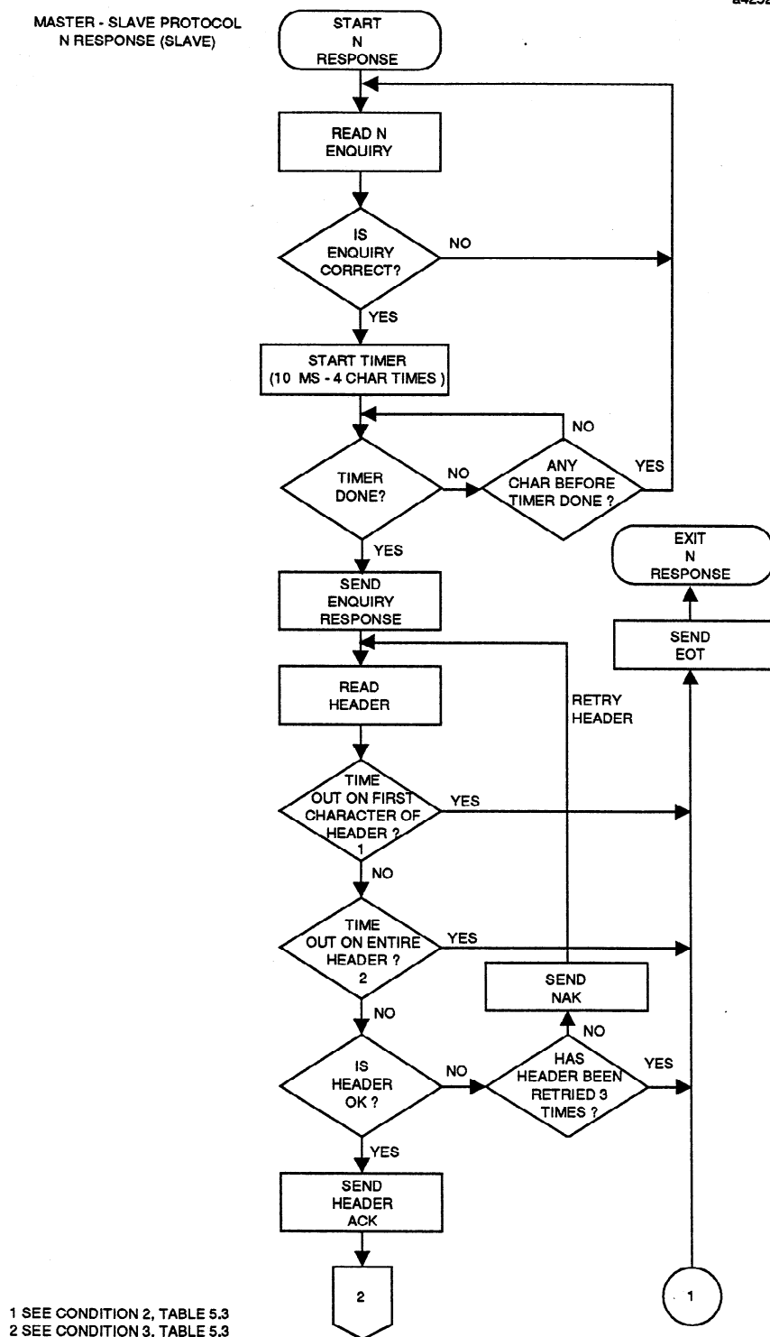
Figure 5-6. N Response, Slave
