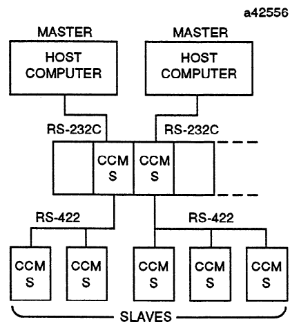
Figure 2-19. Complex Networks (Multiple Hosts)
