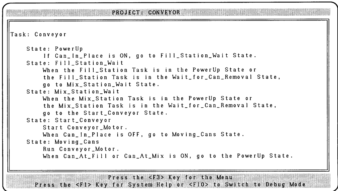
Figure 4-4. Conveyor Task
