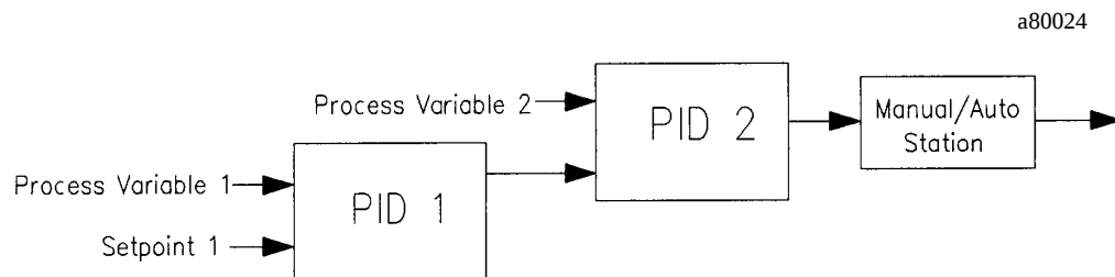
Figure 8-2. Cascaded PID Loops
