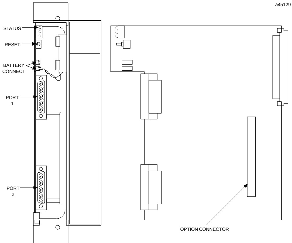
Figure 5-2. Series 90-70 Diagnostic Processor
