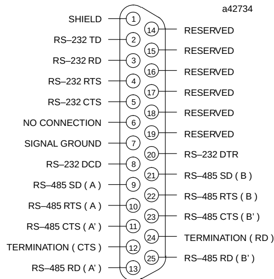
Figure 5-6. Serial Port Assignments for Series 90-70 Diagnostic Processor
