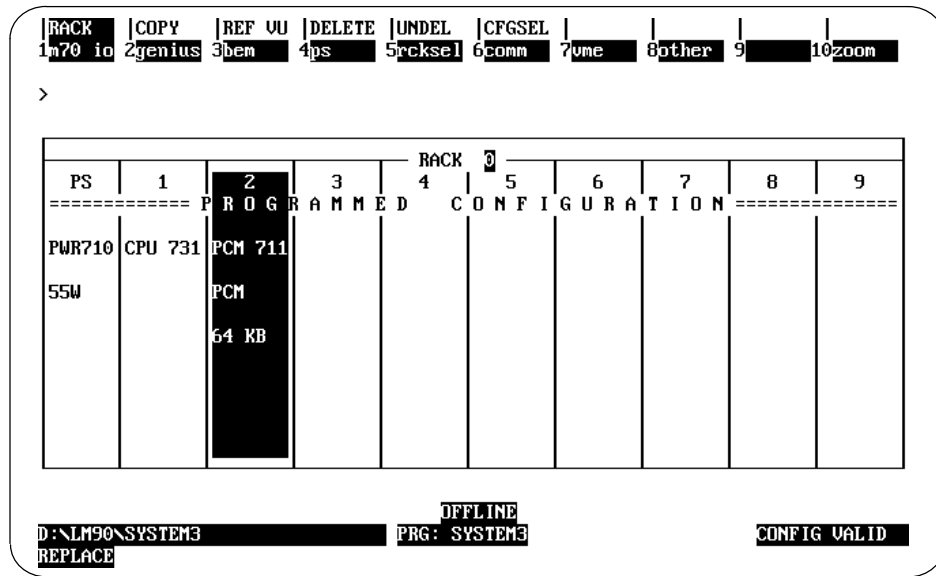
Figure 5-3. Sample Logicmaster Configuration Screen
