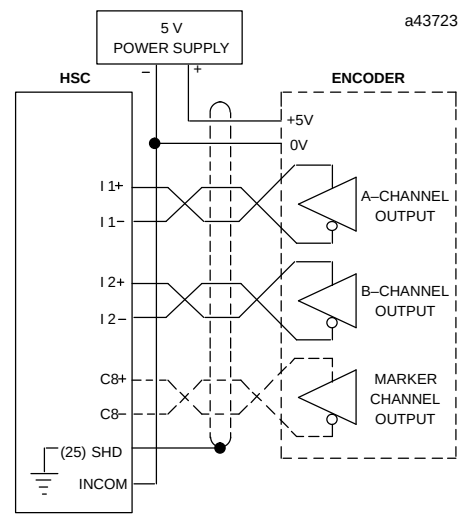
Connections for Differential Inputs Power: Positive Loop
