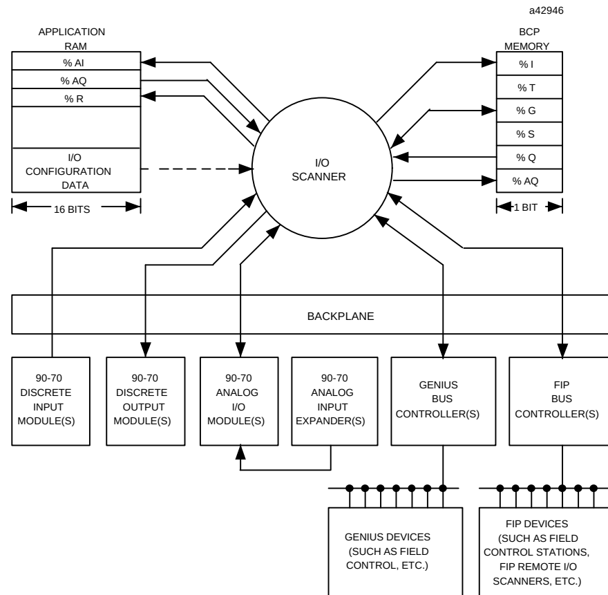
Figure 2-13. Series 90-70 PLC I/O Structure
