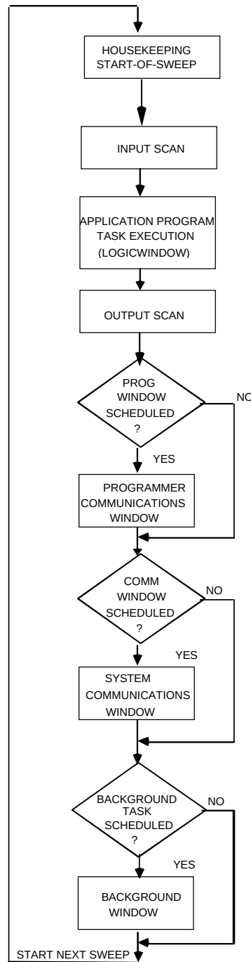
Figure 2-1. Phases of a Typical PLC Sweep
