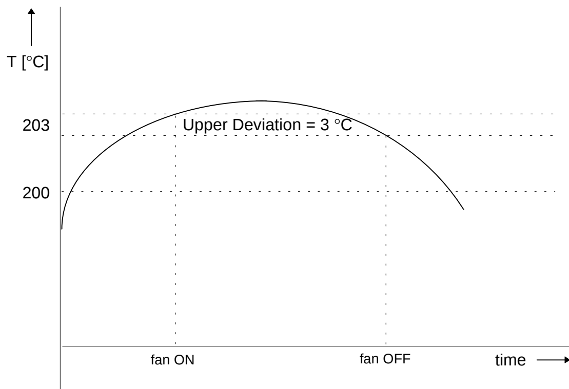
Figure C-1. Heating and Cooling Example 1
