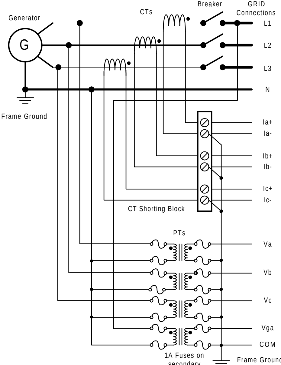
Figure 3-8. Wye Synchro/Power Monitor connection
