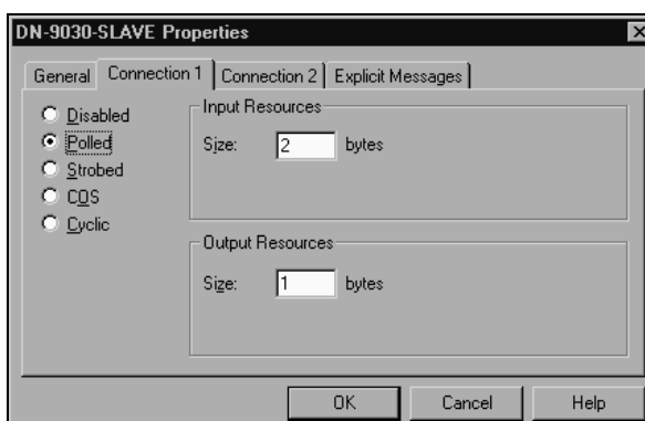
Polled I/O Messaging Screen for a Series 90-30 DeviceNet Slave Module
