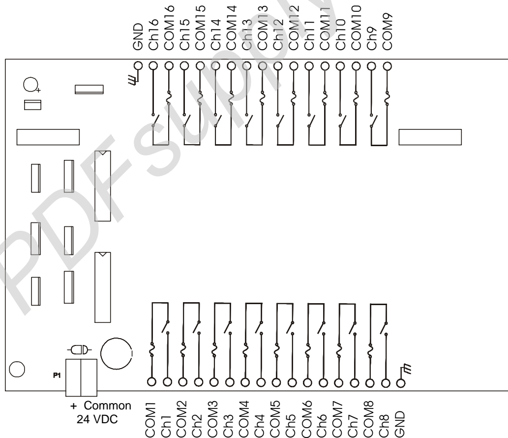
Figure 2 - Top View
