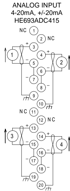
Figure 4 – HE693ADC415 Wiring
