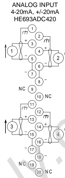
Figure 5 – HE693ADC420 Wiring
