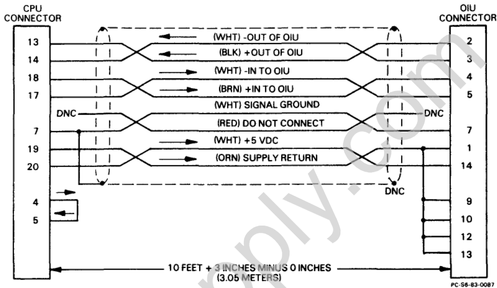
FIGURE 3. WIRING DIAGRAM OF CABLE
