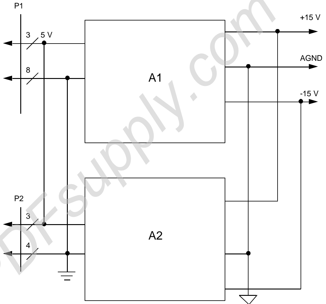
Figure 4-6: DC-to-DC Converters
