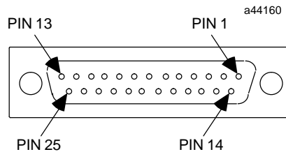
Figure 3-6. Secondary Port Using DB-25S Female Connector
