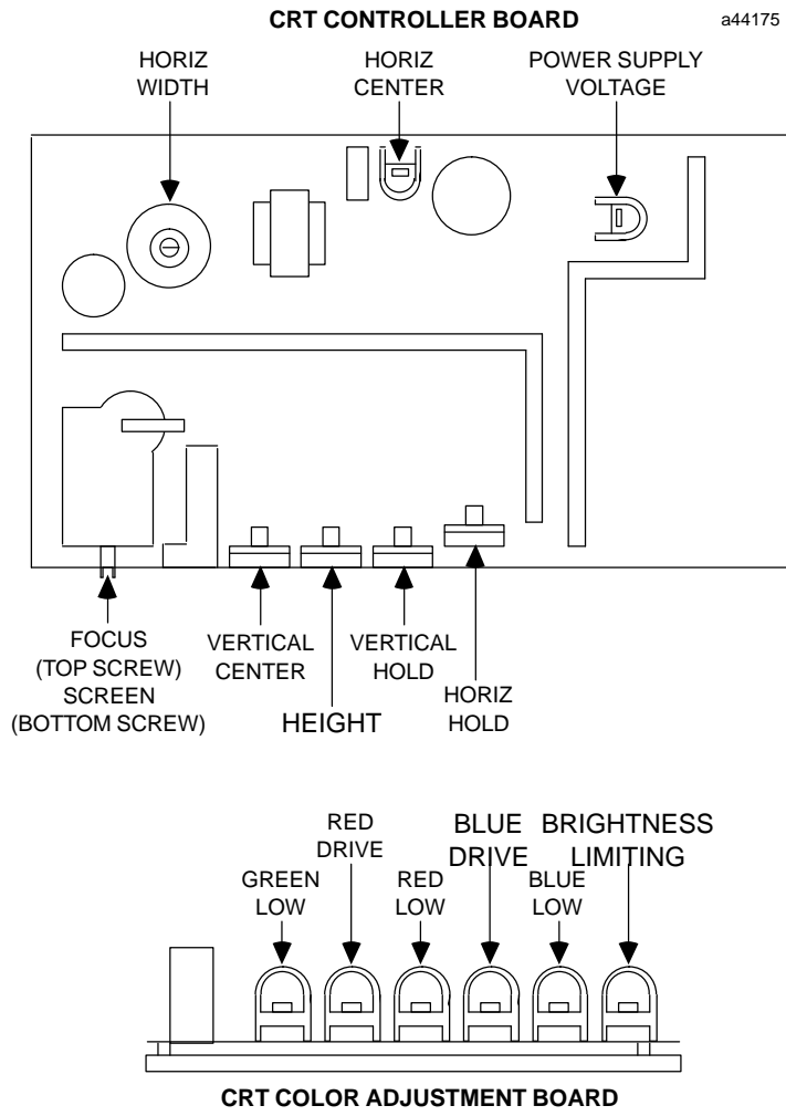
Figure 3-21. Color CRT Adjustment Controls
