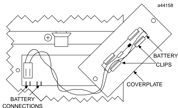
Figure 3-4. Connecting the Battery
