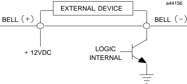
Figure 3-2. Bell Output Wiring
