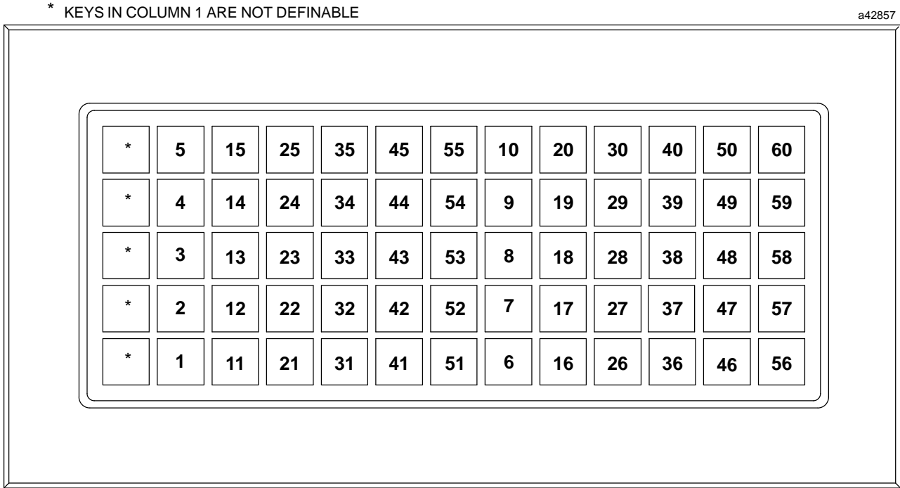
Figure 5-1. Key Location Numbers for the 65-Position Sealed Membrane Keyboard
