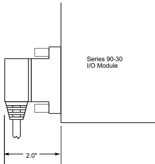
Figure 10-41. Dimension for Depth of Connector
