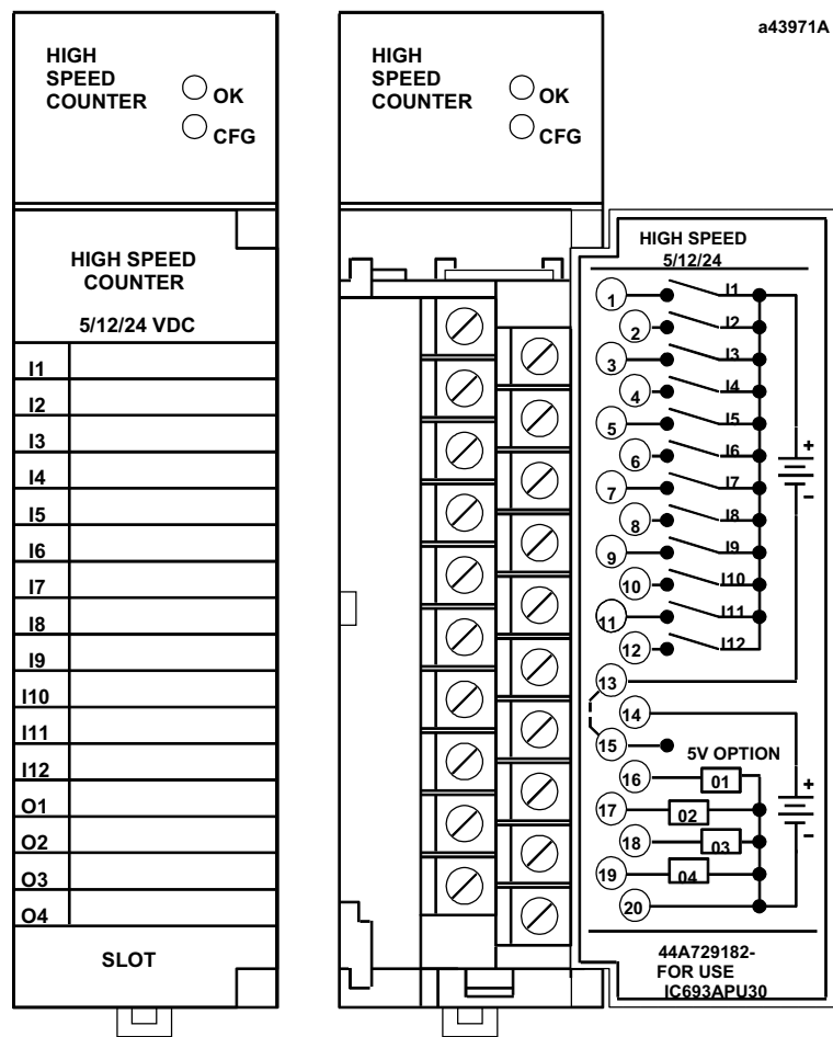
Figure 8-14. High Speed Counter (HSC)
