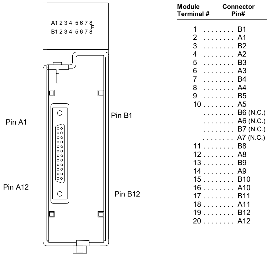
Connector Pin Orientation
