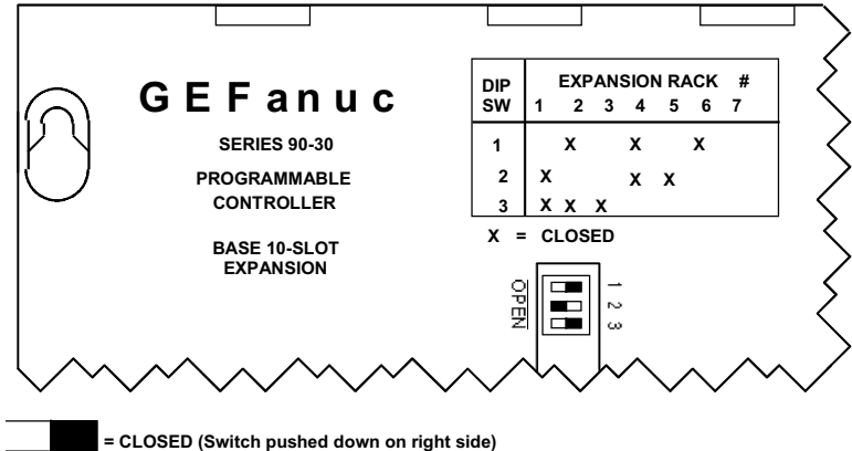
Figure 3-11. Rack Number Selection Switch (Shown with Rack 2 Selected)
