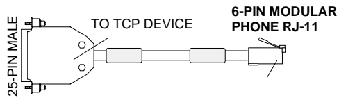
HMI-CAB-C112
