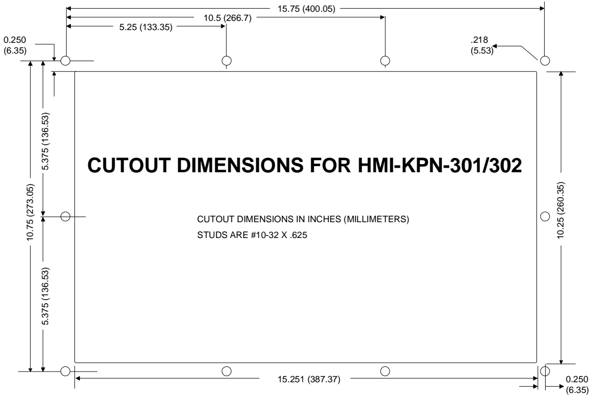
PANEL CUTOUT FOR HMI-KPN-301 and HMI-KPN-302 (9" and 10.5" displays)
