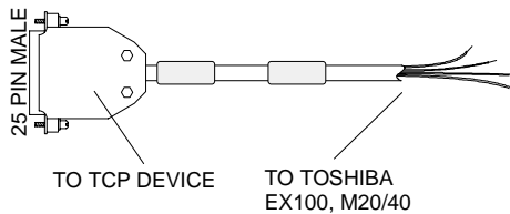
HMI-CAB-C96
