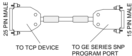
HMI-CAB-C82
