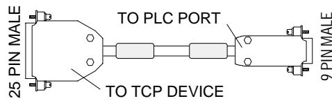
HMI-CAB-C58
