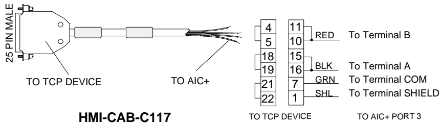
HMI-CAB-C117
