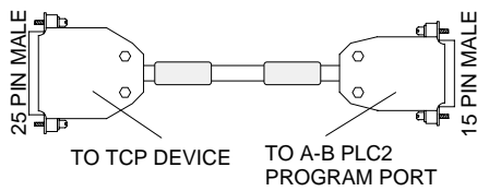
HMI-CAB-C90
