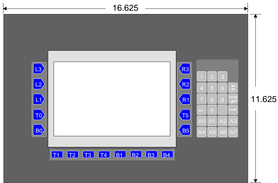
DIMENSIONS FOR HMI-KPN-301/302 (9" and 10.5" displays)
