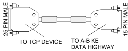
HMI-CAB-C55
