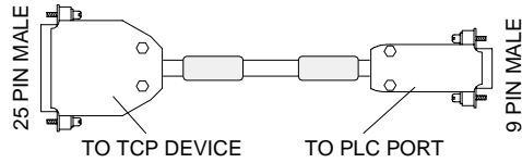
HMI-CAB-C92
