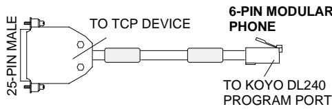
HMI-CAB-C86/B
