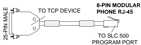
HMI-CAB-C83/A
