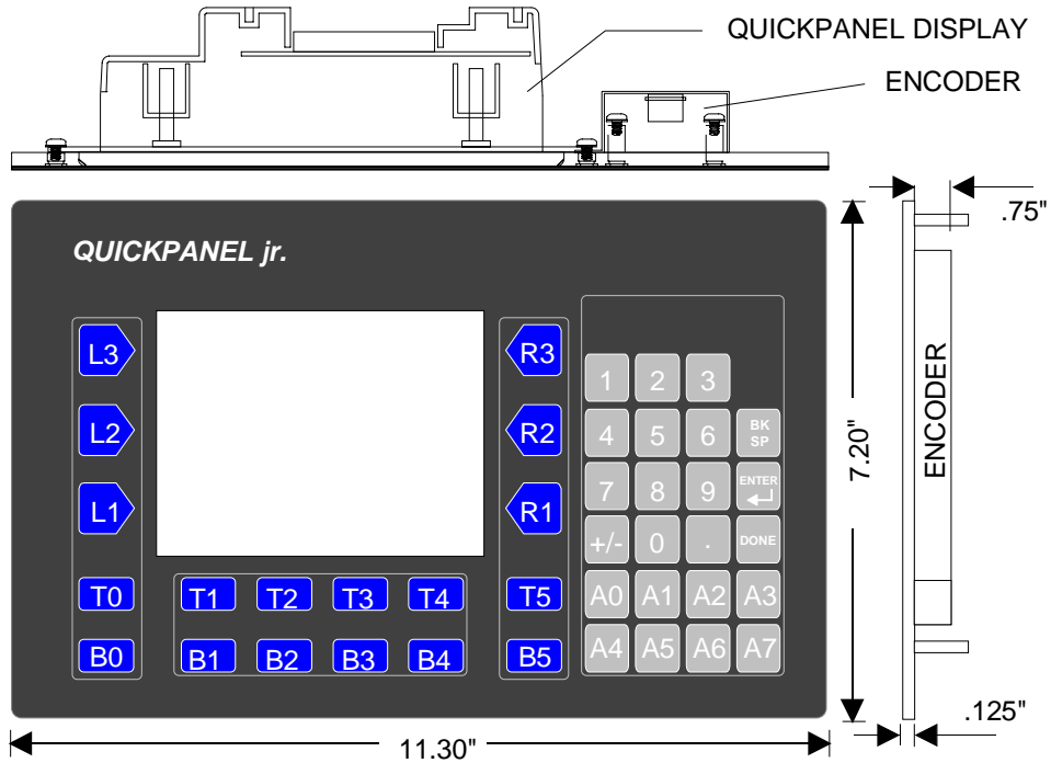
DIMENSIONS FOR HMI-KPN-201 (5" and 6" displays)
