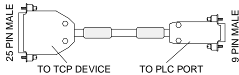
HMI-CAB-C67
