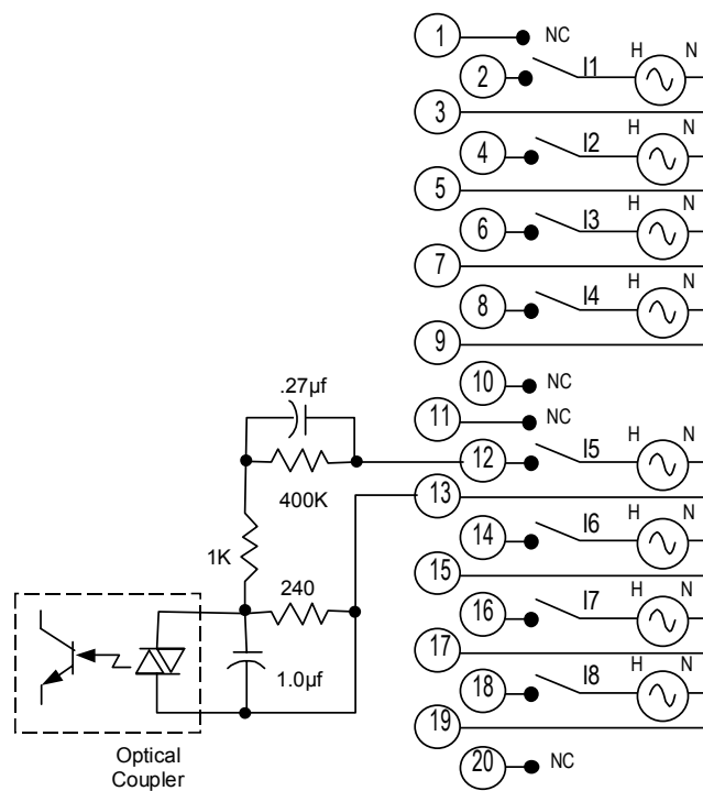
Field Wiring
