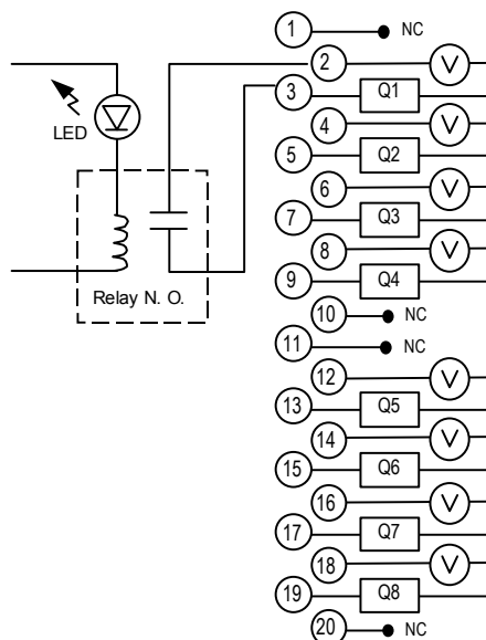
Module Circuits Terminals Field Wiring
