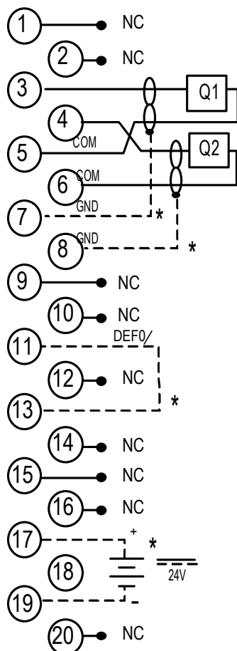
Terminals Field Wiring
