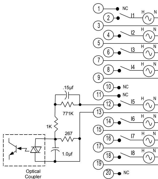
Field Wiring
