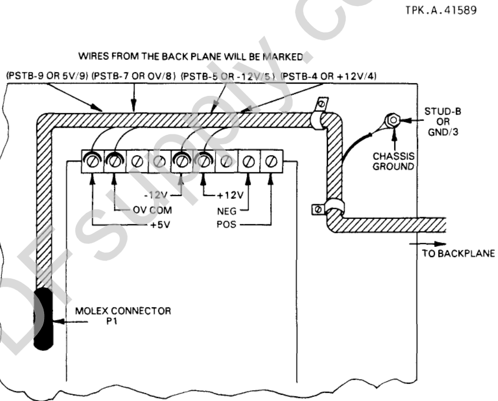
Figure 2 HIGH CAPACITY I/O POWER SUPPLY FRONT PANEL TERMINAL BLOCK
