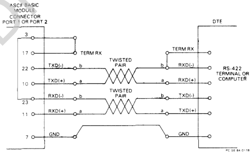
FIGURE 4(c). ASYNCHRONOUS RS-422 POINT-TO-POINT
