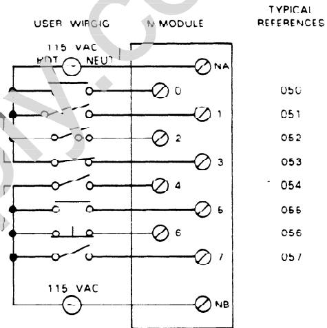
WIRING DIAGRAM
