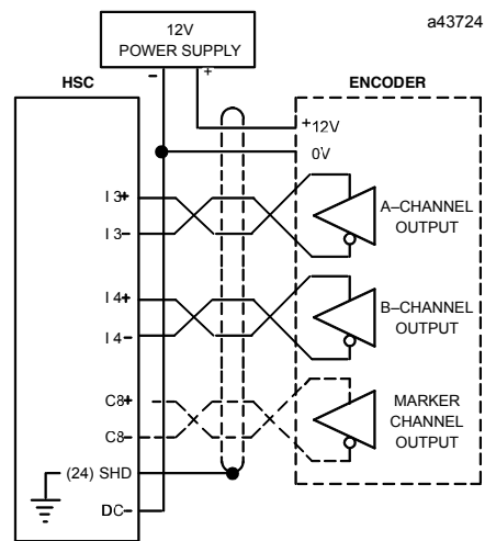
Encoder Wiring in Differential Configuration: Negative Loop
