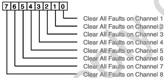
Output Command Bits to Clear Alarms (byte 0)
