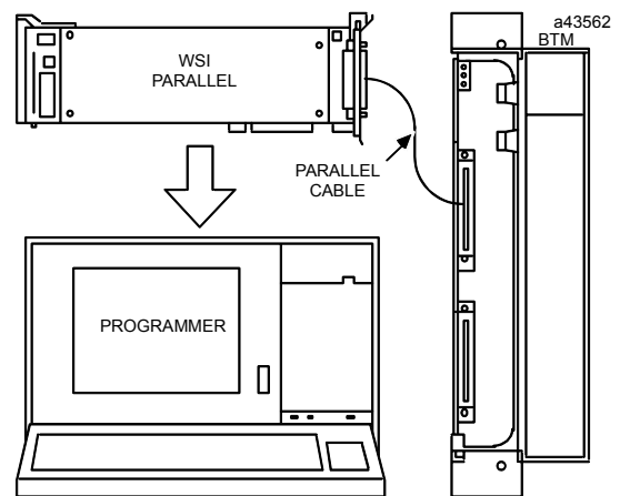
Figure 2. Parallel Programmer Attachment to BTM
