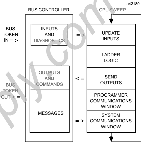
Figure 4. CPU Sweep
