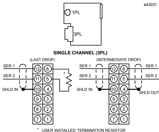
Figure 5. Wiring Diagram
