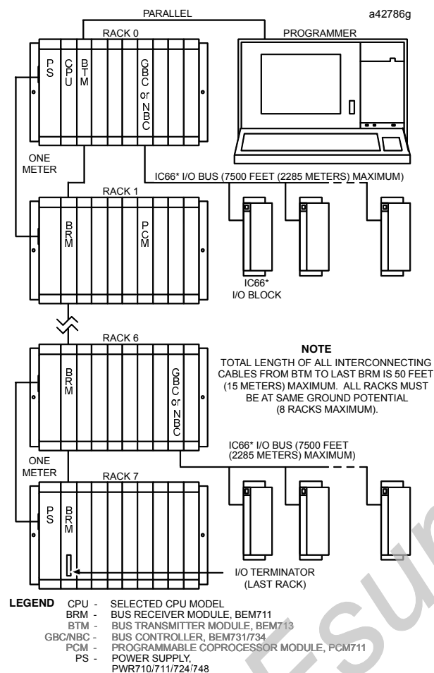
Figure 1. Typical Programmable Controller System Configuration
