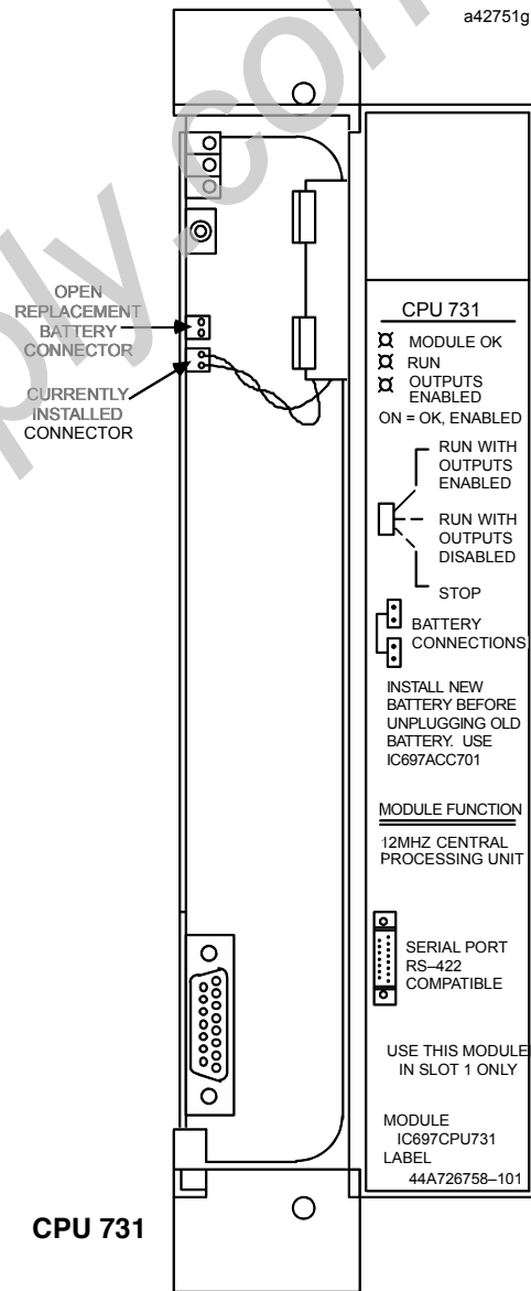
Figure 2. CPU 731- Location of Major Features
