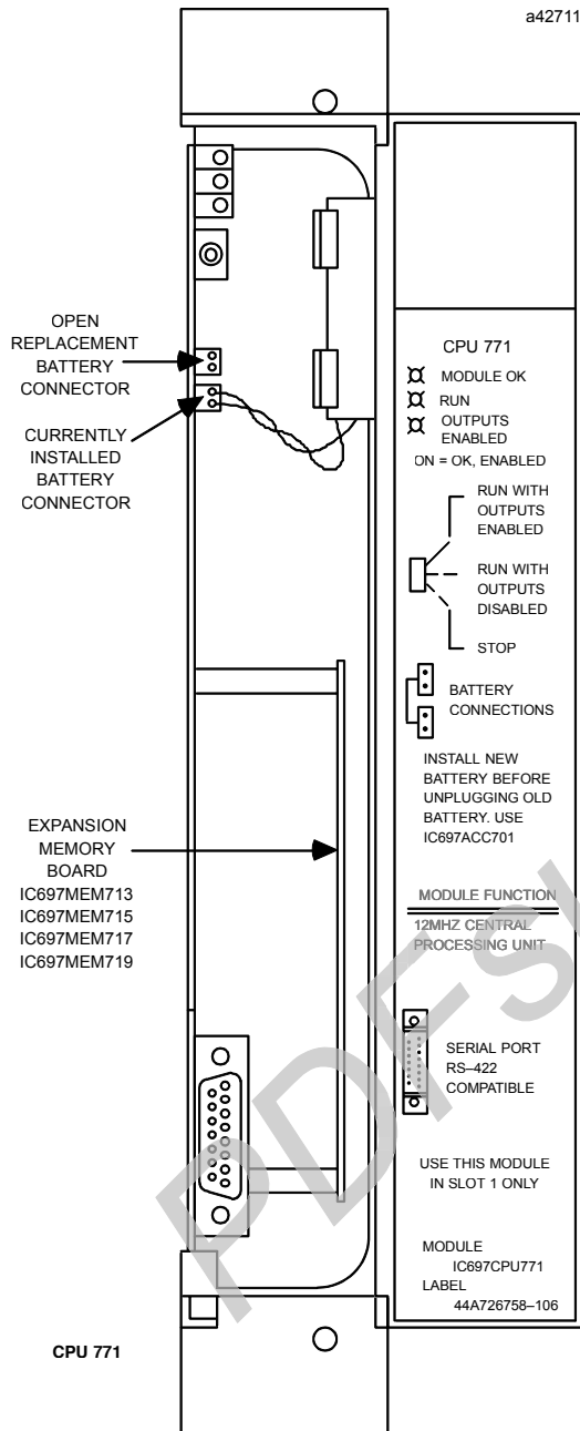
Figure 2. CPU 771 - Location of Major Features
