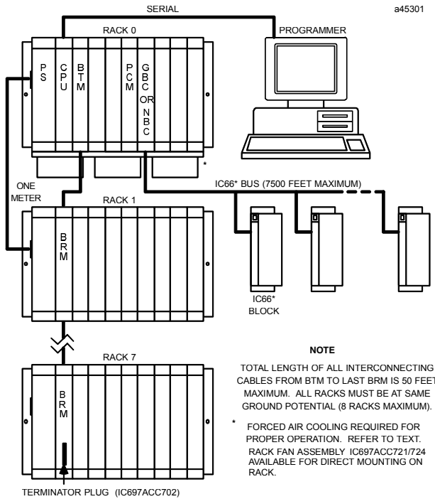
Figure 3. System Configuration, Serial Connection to Programmer
